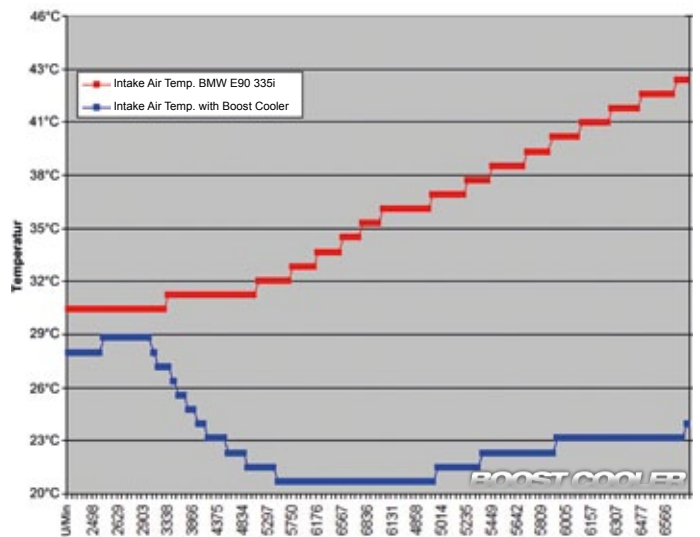
Example Diagram: Boost Cooler-Intercooling
