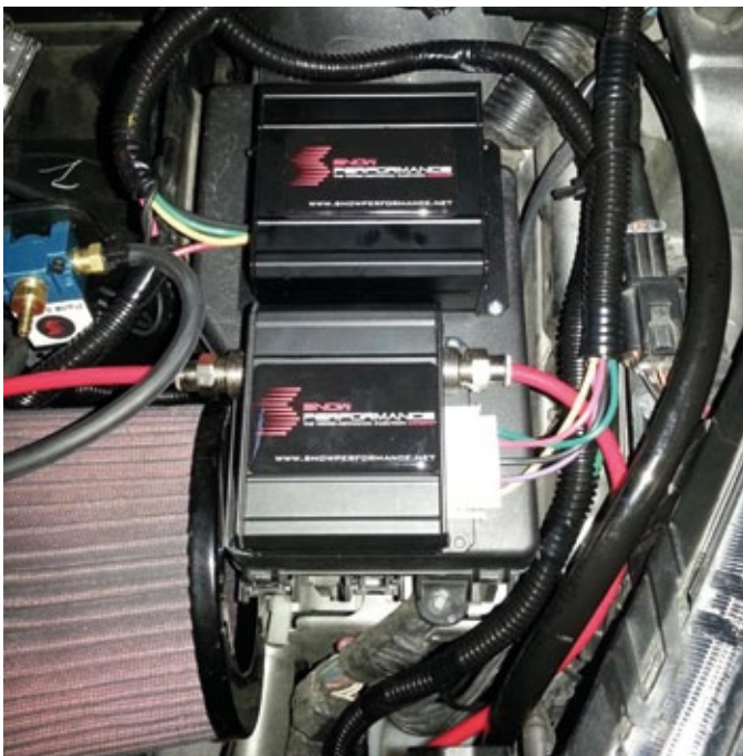
SafeInjection- and Stage 2 Controller in the engine compartment (Mazda 3 MPS)
